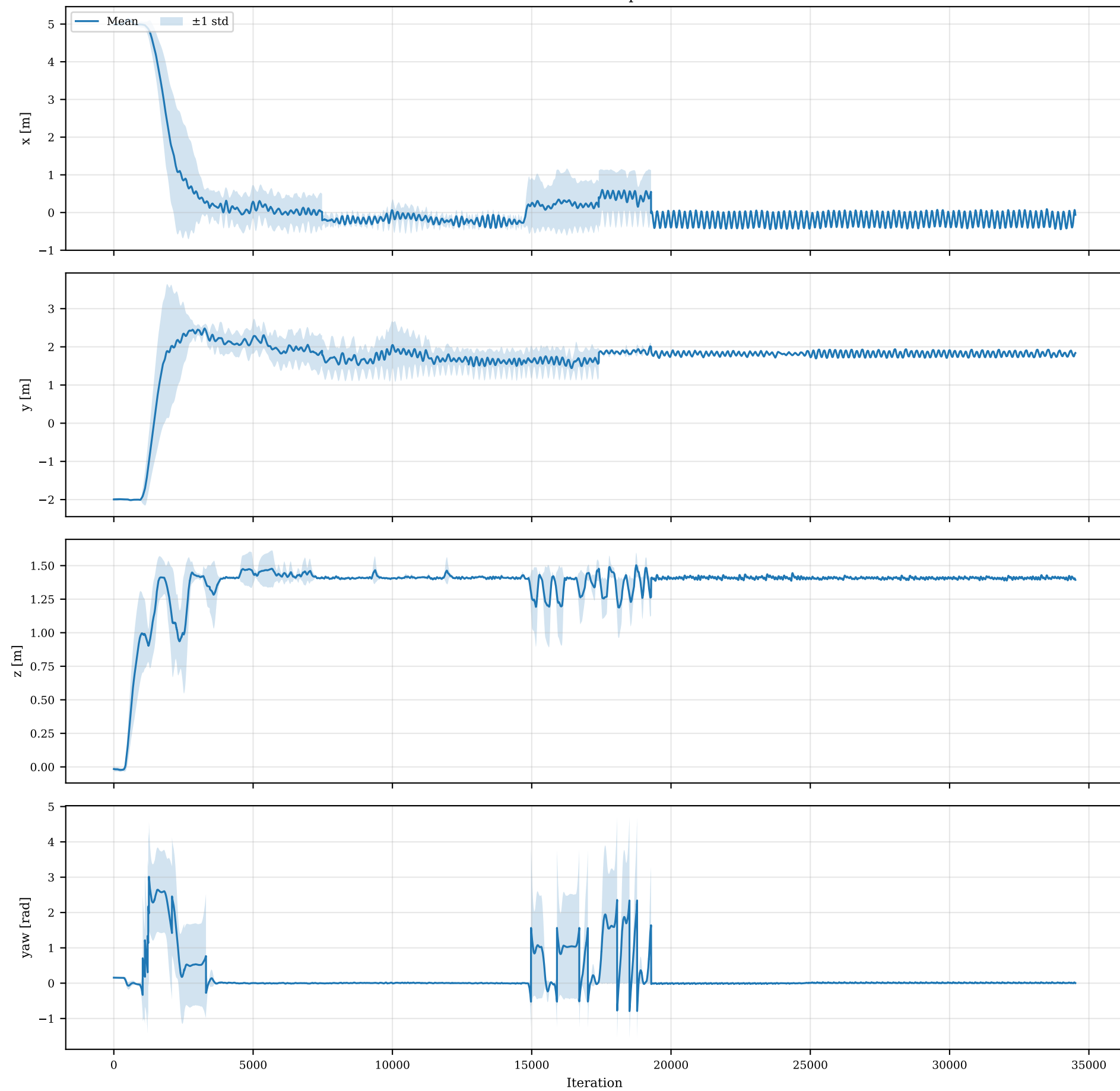
Normal APF - UAV 30 - Mean position \pm std
